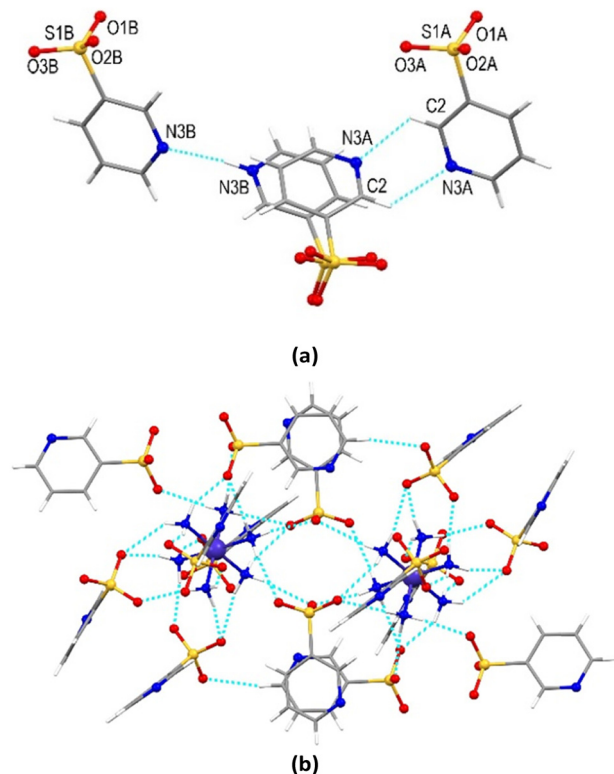
Fig. 1 (a) The H-bonds between the disordered pyp - anions and the neutral Hpyp molecule in 1 . (b) H-bonding interactions around [Co(NH 3 ) 6 ] 3+ cations in the structure of 1 . Hydrogen bonds are shown as blue dashed lines.
