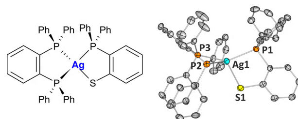
Fig. 1 Left: Schematic drawing of the [Ag(dppbz)(dpps)] complex ( AgPPPS ). Right: Molecular structure of AgPPPS in the solid state. Thermal motion is shown as ellipsoids (50% probability), and labelling of carbon atoms and all hydrogen atoms are omitted for clarity.
