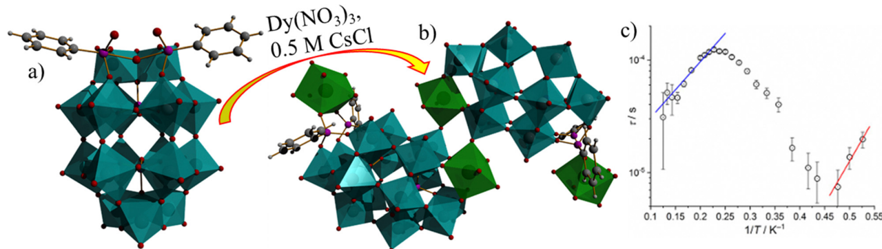
Fig. 11 The structure of the building unit, [a_2\text{-P}_2\text{W}_{17}(\text{PhPO})_2]^{6-} (a), the molecular structure of \{[(\text{H}_2\text{O})_7\text{Dy}_2(a_2, a_2'\text{-P}_2\text{W}_{16}\text{O}_{60})(\text{PhPO})_2]_2\}^{8-} (b), and magnetic relaxation plot of the complex (c). Color code: cyan octahedron ( \text{WO}_6 ), green polyhedral Dy, red O, pink P, grey C, white H. Pictures reproduced from ref. 150 with permission from the Royal Society of Chemistry.
