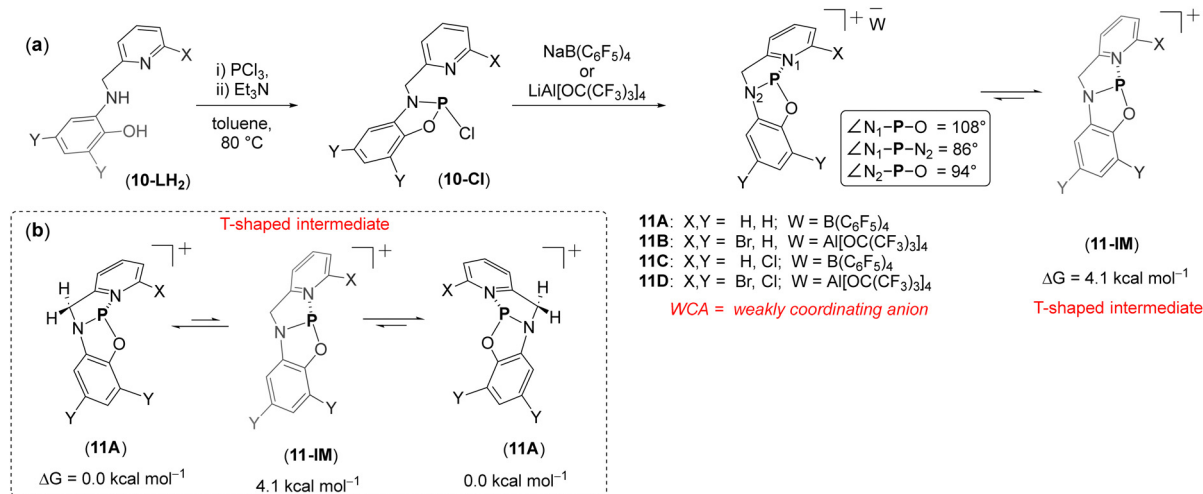
Fig. 6 Synthetic scheme for the synthesis of (a) [11][\text{W}] ; (b) isomerization between bent structures of 11 via a T-shaped planar structure.
