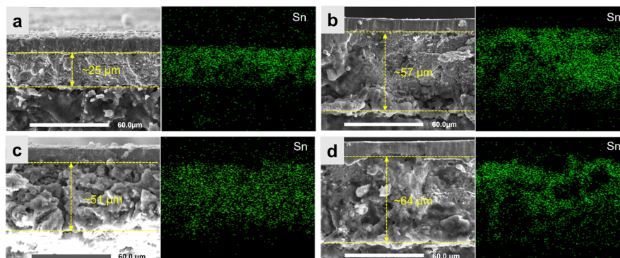
Fig. 4 Thickness of LiSn anodes under different states. (a) Initial, (b) charging, (c) discharging, and (d) after 50 cycles.
