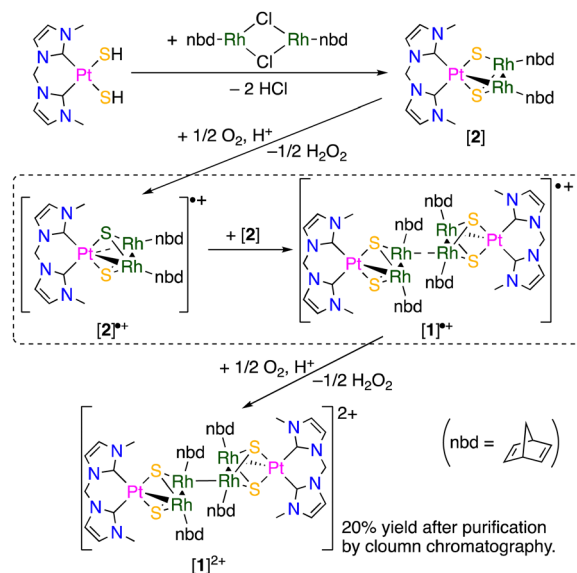
Scheme 2 Formation and oxidative coupling of trinuclear precursor [2] affording hexanuclear cluster [1]^{2+} via the formation of one-electron oxidised trinuclear intermediate [2]^{\bullet+} and hexanuclear precursor [1]^{\bullet+} .
