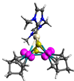
Fig. 4 Spin density of [2]^{\bullet+} (magenta). Pt: beige, Rh: green, S: yellow, N: blue, C: grey and H: white.
