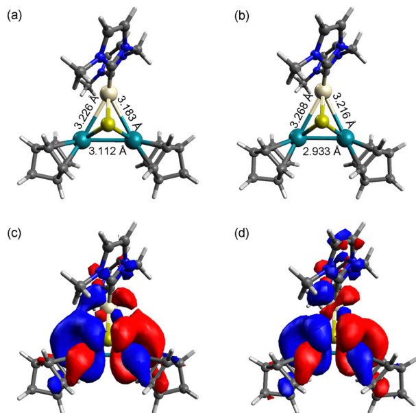
Fig. 3 Optimised structures of (a) 48-CVE complex [2], (b) one-electron oxidised complex radical [2]^{\bullet+} , (c) HOMO of [2] and (d) SOMO of [2]^{\bullet+} . Pt: beige, Rh: green, S: yellow, N: blue, C: grey and H: white.
