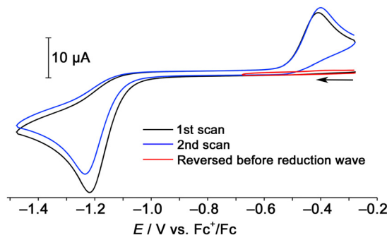
Fig. 5 Cyclic voltammograms of [1]\text{Cl}_2 in \text{CH}_3\text{CN} with 0.10 \text{ mol L}^{-1} of n\text{Bu}_4\text{NPF}_6 (Scan rate: 100 \text{ mV s}^{-1} ).
