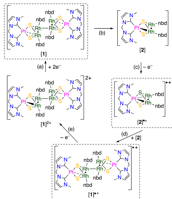
Scheme 3 ECECE process on reduction and reoxidation scans of [1]\text{Cl}_2 : (a) two-electron reduction affording a neutral hexanuclear complex, (b) subsequent reaction giving trinuclear 48-CVE complex [2], (c) reoxidation of the 48-CVE complex affording the complex radical [2]^{\bullet+} , (d) reaction of [2]^{\bullet+} with [2] and (e) reformation of [1]^{2+} by one-electron oxidation of [1]^{\bullet+} .
