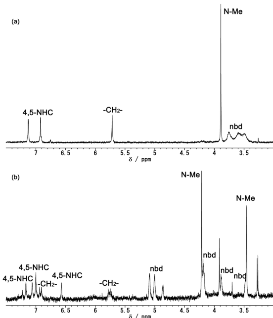
Fig. 6 ^1\text{H} NMR spectra of the reaction mixture of [1]\text{Cl}_2 and 2 eq. of decaethylcobaltocene (a) under an inert atmosphere and (b) after exposing to air. ( \text{CD}_3\text{CN} , 400 MHz, 293 K) (see Fig. S8 in ESI† for the whole spectra).
