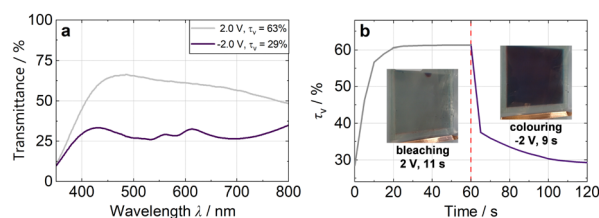
Fig. 5 (a) Spectroelectrochemical characterization and (b) switching time determination of the Red1/PB2 ECD at cell voltage \pm 2 \text{ V} .
