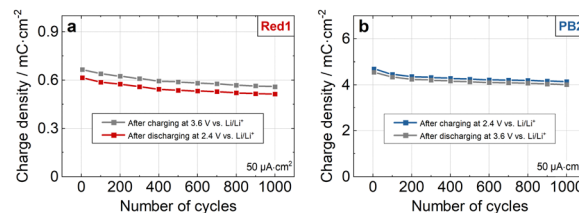
Fig. 4 Charge/discharge measurements over 1000 switching cycles for (a) Red1 and (b) PB2 , performed at 50 \mu\text{A cm}^{-2} .
