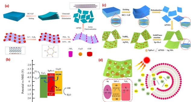
Fig. 18 (a) Synthesis scheme of Ti 3 C 2 /TpPa-1/Cu 2 O; (b) proposed mechanism, reprinted with permission from ref. 45. Copyright 2022 Elsevier; (c) synthesis scheme of Ti 3 C 2 /TpPa-1/Ag; and (d) proposed antibacterial mechanism. Reprinted with permission from ref. 46. Copyright 2023 Elsevier.
