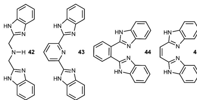
Fig. 12 Ligands used in combination with RuCl 3 ·3H 2 O for the catalytic ethanol upgradation studied by Jones and co-workers. 97a
