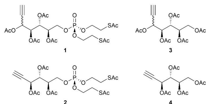
Figure 2. Structures of alkyne-tagged ribitol and Rbo5P derivatives synthesised in this study for the metabolic labelling of Rbo5P-containing glycans.
