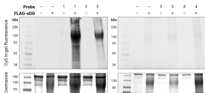
Figure 3. Metabolic labelling of \alpha -DG in mammalian cells. PiggyBac transposon-generated HEK293F cells expressing FLAG-tagged \alpha -DG were induced with doxycycline and treated with 200 \mu M of probes 1–4 for 34 hours. Media were collected and immunoprecipitated with anti-FLAG resin. Click reaction was performed on-resin with Cy5-picolyl azide, after which proteins were eluted, resolved on SDS-PAGE and detected by in-gel fluorescence (top) and Coomassie staining (bottom). Non-induced cells ('- FLAG- \alpha -DG') and non-probe treated cells ('- probe') were included as controls.
