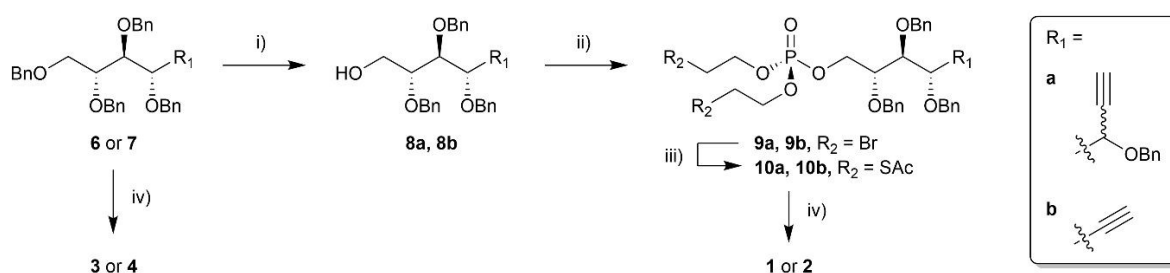
Scheme 2. Synthesis of target probes 1-4 . i) \text{ZnCl}_2 , \text{Ac}_2\text{O} , \text{AcOH} , 0^\circ\text{C} -rt; then \text{K}_2\text{CO}_3 , \text{MeOH} , rt, 8a : 71% (dr 3:1), 8b : 68% over two steps. ii) \text{OP}(\text{OCH}_2\text{CH}_2\text{Br})_3 , \text{Trf}_2\text{O} , pyridine, \text{CH}_2\text{Cl}_2 , rt, 9a : 65% (dr 3:1), 9b : 57%. iii) \text{KSAC} , pyridine, rt, 10a : quantitative (dr 3:1), 10b : quantitative. iv) \text{BCl}_3 , \text{CH}_2\text{Cl}_2 , -78^\circ\text{C} ; then \text{Ac}_2\text{O} , pyridine, rt, 1 : 31% (dr 7:1), 2 : 34%, 3 : 85% (dr 10:1), 4 : 57% over two steps.
