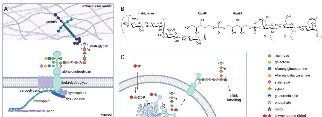
Figure 1. A chemical reporter strategy to interrogate glycosylation of the mammalian protein \alpha -dystroglycan ( \alpha -DG). A) O-mannosylation of \alpha -DG, in particular formation of core M3 glycans carrying the matriglycan motif, is essential for the laminin-binding function of the dystrophin-glycoprotein complex. B) Structure of a core M3 glycan fully extended with matriglycan and containing two tandem ribitol-5-phosphate (Rbo5P) residues. C) Metabolic glycan engineering with tagged Rbo5P derivatives. Upon cellular uptake, the probes are metabolically converted into cytidine diphosphate (CDP)-activated glycosylation donors and incorporated into core M3 glycans on \alpha -DG.
