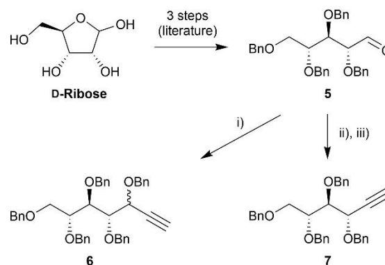
Scheme 1. Synthesis of alkyne-tagged probe scaffolds. i) ethylmagnesium bromide, TMS-acetylene, THF, -78^{\circ}\text{C} -rt; then NaH, BnBr, THF, 0^{\circ}\text{C} -rt, 58% over two steps (dr 3.5:1). ii) \text{CBr}_4 , \text{PPh}_3 , \text{Et}_3\text{N} , \text{CH}_2\text{Cl}_2 , -10^{\circ}\text{C} -rt, 84%. iii) LDA, THF, 72%.
