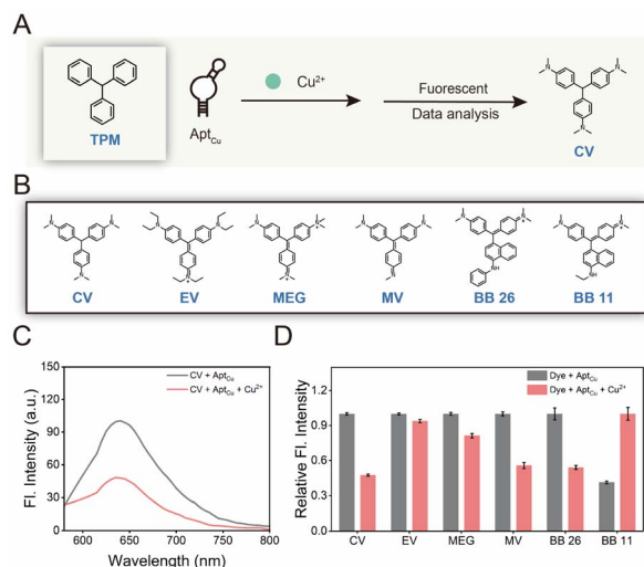
Fig. 1 (A) Screening of fluorescent dyes from the TPM dye library for their ability to bind to the aptamer and \text{Cu}^{2+} . (B) Chemical formulae of six selected TPM dyes. (C) Fluorescence spectra of CV dye in the presence or absence of \text{Cu}^{2+} in solution. (D) Relative fluorescence of the TPM dyes/Apt Cu with or without \text{Cu}^{2+} .
