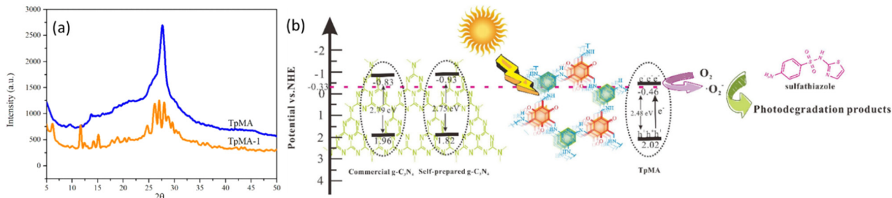
Fig. 17 (a) XRD spectra of the ball-milled material (TpMA) and the solvothermally prepared one (TpMA-1). (b) Band structures of commercial g\text{-C}_3\text{N}_4 , self-prepared g\text{-C}_3\text{N}_4 and TpMA, and the mechanism of photo-degradation of sulfathiazole catalysed by TpMA. Adapted with permission from ref. 186. Copyright 2021 Elsevier.
