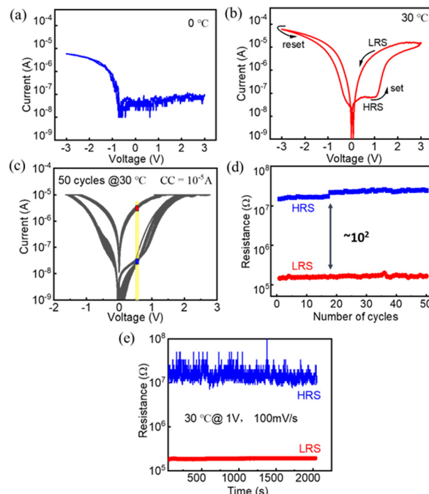
Fig. 2 Typical I - V curves of a Ag/ [\text{C}_{12}\text{mim}][\text{BF}_4] /H:Si(100) device at (a) 0 °C and (b) 30 °C. (c) I - V curves in 50 consecutive voltage sweep cycles with a compliance current (CC) of 10^{-5} A at 30 °C. (d) Endurance characteristics of the device, where the resistance values in the HRS and LRS measured from (c) at 0.5 V (yellow line) are plotted, respectively, against the number of cycles. (e) Retention characteristics of the device, where the resistance values of the HRS and LRS measured at +1 V are plotted as a function of time.
