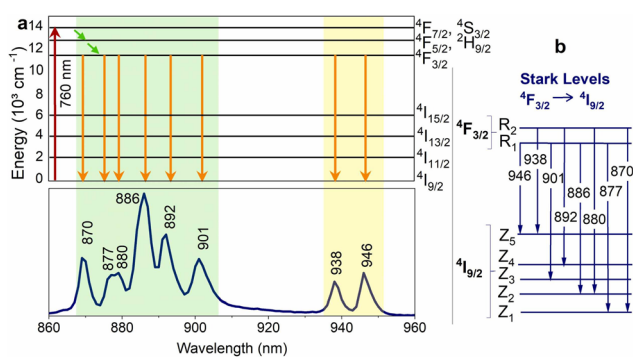
Fig. 3 (a) \text{Nd}^{3+} partial energy level diagram illustrating the excitation (760 nm) and relaxation pathways. The bottom part of the figure shows the corresponding emission spectrum of \text{Y}_3\text{Al}_5\text{O}_{12}:\text{Nd}^{3+} NPs. (b) Representation of the Stark levels of the \text{Nd}^{3+} manifolds {}^4\text{F}_{3/2} and {}^4\text{I}_{9/2} , as well as the electronic transitions associated with the emission peaks in the lower part of Fig. 3a. 82
