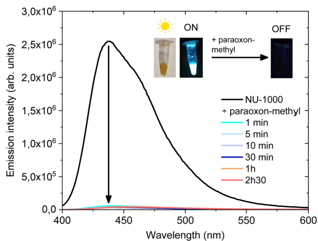
Fig. 6 NU-1000 emission spectra at \lambda_{\text{ex}} = 385 nm recorded at different times during the degradation of paraoxon-methyl (1 mL of 1.3 mM NU-1000, 4 \mu L of paraoxon-methyl, 500 \times dilution prior to analysis).
