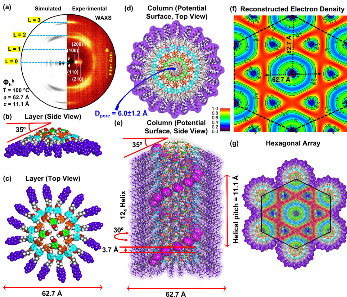
Fig. 4 X-ray diffraction analysis and molecular models of at 100 °C ( \Phi_{\text{h}}^{\text{k}} phase). (a) Wide-angle fiber XRD patterns (WAXS) and simulated XRD patterns from the molecular model showing the similarity; (b) formation of the layer by four molecules showing the tilt angle (side view); (c) layer with four molecules (top view); (d) formation of the column by repeat of the tetramer layer (potential surface, side view); (e) column (potential surface, top view); (f) reconstructed relative electron density map; (g) hexagonal array by the columns (potential surface; top view). Color codes used in the molecular models are similar as shown in the ChemDraw structure of 14 . O atoms, red; H atoms, white; F atoms, purple; C atoms in the phenyl rings connected apex –CO 2 CH 3 group, green; C atoms in the phenyl rings connected of the first generation, orange; C atoms in other phenyl rings in the second generation, light blue; all other C atoms, grey. Potential surface is in fact the “van der Waals surface” and the color codes for the potential surface are similar as the colors of the atoms; transparency (50%) was added for clarity.
