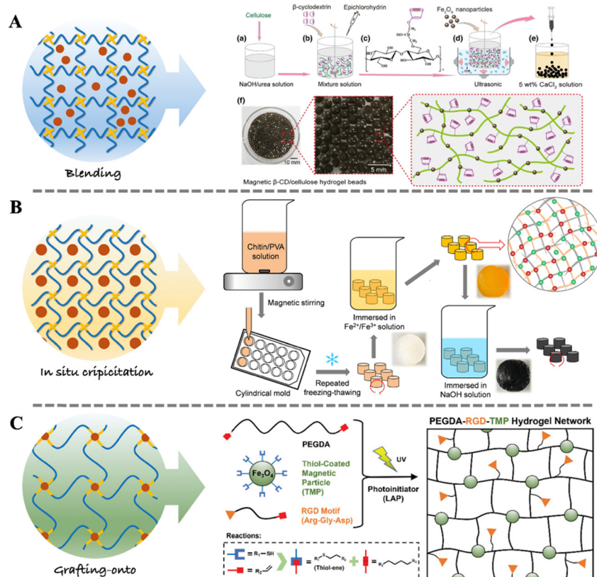
Fig. 2 Fabrication strategy of magneto-responsive biocomposites. (A) Schematic steps for the synthesis of magnetic β-CD/cellulose hydrogel using the blending method. 84 Copyright 2019, Springer Netherlands. (B) Schematic steps for the synthesis of chitin/PVA-based magnetic hydrogel using the in situ precipitation method. 85 Copyright 2019, Elsevier. (C) Schematic steps for the synthesis of PEGDA-RGD-TMP hydrogel using the grafting-onto method. 43 Copyright 2023, Wiley.
