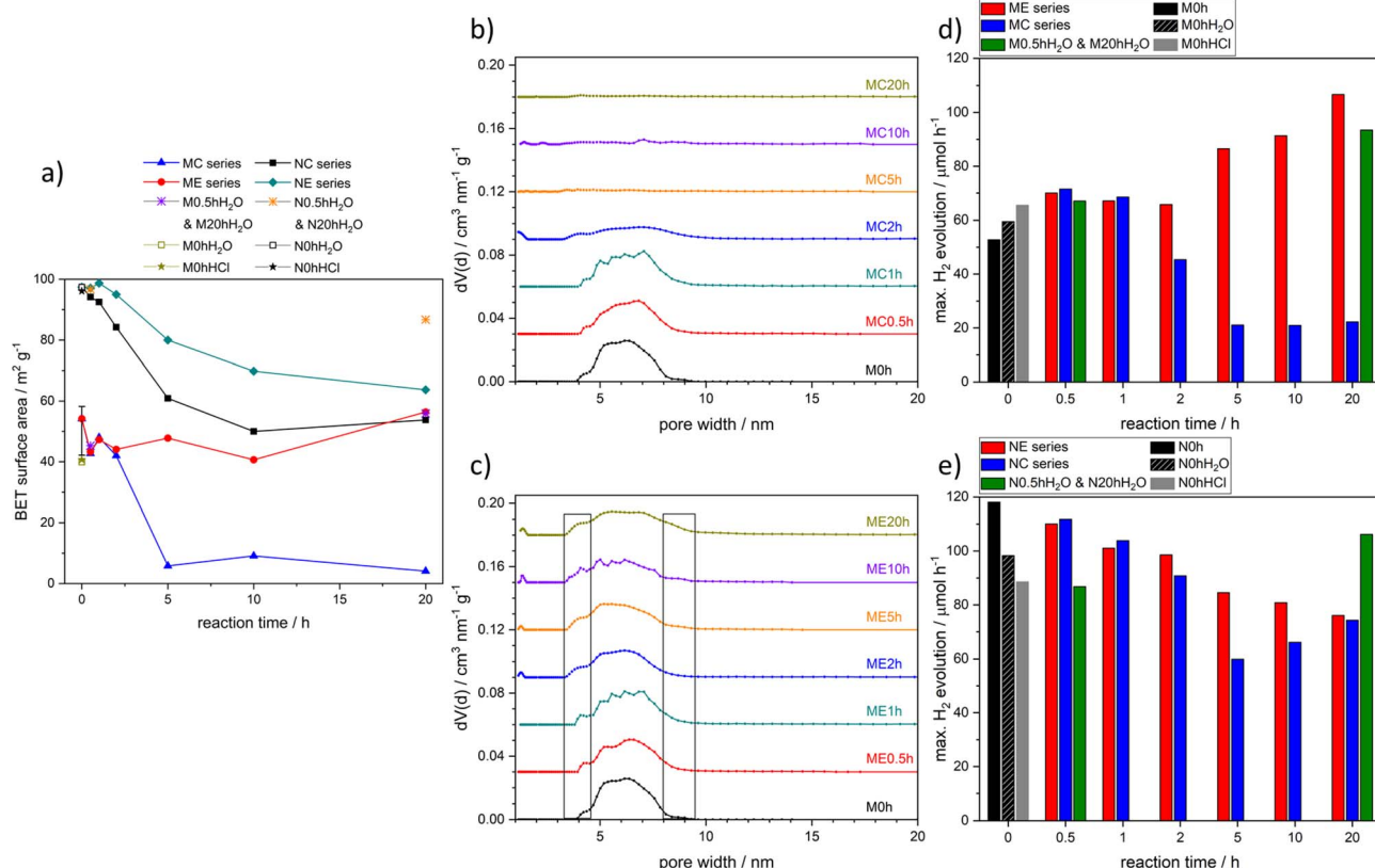
Fig. 5 BET surface areas (a), pore size distributions (each shifted by 0.03 \text{ cm}^3 \text{ nm}^{-1} \text{ g}^{-1} ) of the MC (b) and ME series (c), and maximum photocatalytic \text{H}_2 evolution rates of all mesoporous (d) and nanoparticulate samples (e) up to synthesis reaction times of 20 h.
