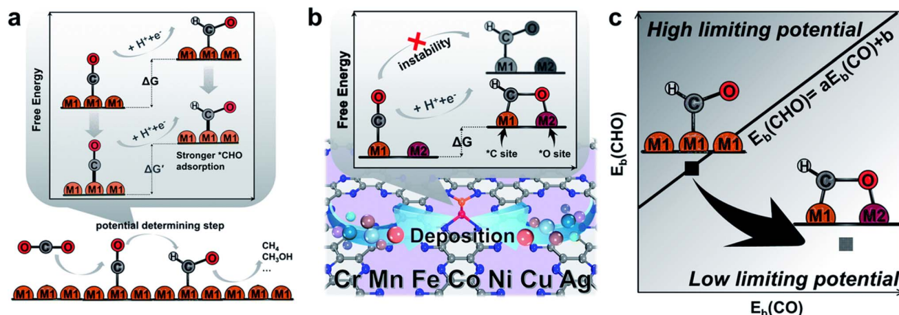
Fig. 1 (a) Effect of free energy change caused by the scaling relations between \text{CO} and \text{CHO} . (b) C 2 N supported heteronuclear transition-metal dimers in stabilizing \text{CHO} . (c) The scaling relations between adsorption energies of \text{CHO} and \text{CO} . 30
