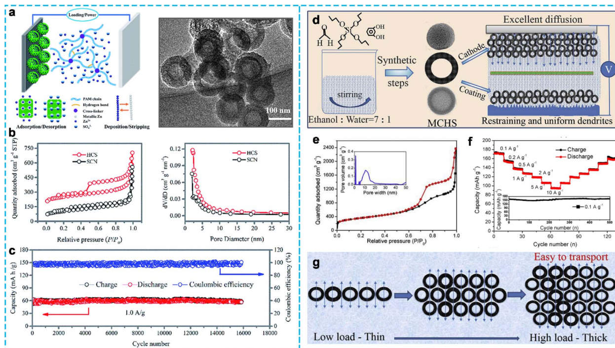
Fig. 7 (a) Schematic illustration of the working principle of the ZHCs and corresponding morphology of HCSs, (b) \text{N}_2 adsorption-desorption isotherms and pore diameter distributions of HCSs, and (c) cycle performance of the HCS cathode at 1.0 \text{ A g}^{-1} . 80 Copyright 2019, The Royal Society of Chemistry. (d) Synthesis process and application of MCHSs, (e) \text{N}_2 sorption isotherms (inset is the pore size distribution), (f) rate performance, and (g) scheme of the ion transport processes in MCHSs with different mass loadings. 82 Copyright 2020, Elsevier.
