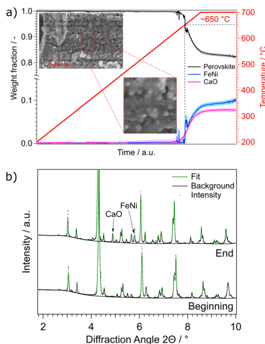
Fig. 6 (a) Weight fractions of NCF-Ni during a reduction ramp. The temperature was increased by a rate of 3 °C \text{min}^{-1} from 200 °C to 700 °C in \text{H}_2/\text{H}_2\text{O} atmosphere. At around 650 °C, a FeNi phase as well as a CaO phase started to form. This indicates the start of the exsolution process as well as the accompanied A-site segregation to compensate for the loss of B-site atoms. SEM images taken after the reduction experiments reveal nanoparticles with a diameter of around 60 nm, consistent with particles observed after reduction at 700 °C in lab-based experiments (Fig. 2c). (b) Comparison between the first and last diffractogram of the reduction. The emerging phases CaO and FeNi are marked.
