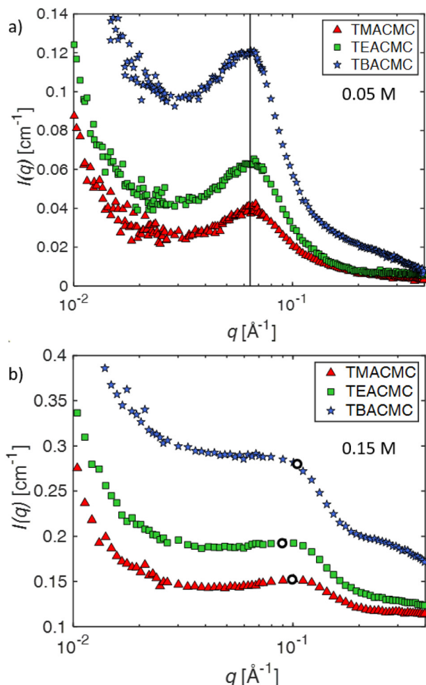
Fig. 3 SANS scattering intensity I as a function of scattering wavevector q for tetra-alkylammonium salts of CMC, see legend for colour scheme. a: c = 0.05 \text{ mol L}^{-1} and b: 0.15 \text{ mol L}^{-1} . The line indicates the position of the peaks at that concentration ( q^* = 0.064 \text{ \AA}^{-1} ). The hollow points represent the peak positions in TMACMC and TEACMC and the scattering plateau position in TBACMC.
