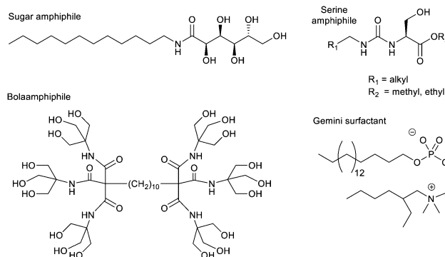
Fig. 10 Selected examples of charge-neutral amphiphile-based gels.
