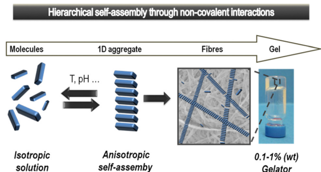
Fig. 1 Schematic of low-molecular-weight gelator (LMWG) assembly from an isotropic solution to anisotropic self-assembled objects that hierarchically assemble further to ultimately form a gel-phase material. Reproduced from ref. 5 with permission from the Royal Society of Chemistry, © 2014.
