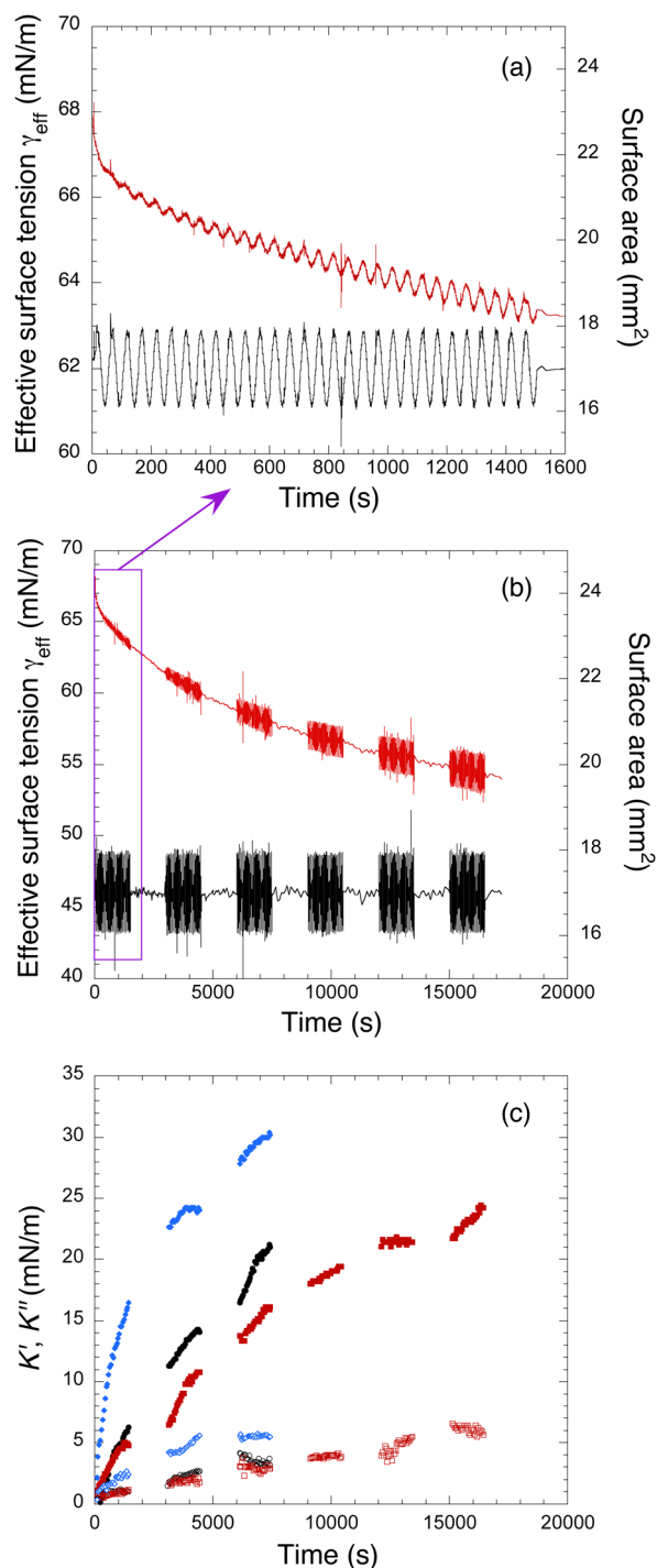
Fig. 3 Dilatometry experiments during the adsorption of the first NaPSS layer, the surface area value being periodically modulated by a sine wave with amplitude \lambda_0 = 0.05 = 5\% and frequency f = 0.02 Hz: (a) zoom on the first 1500 s of the experiment in (b), where we plot the time dependence of effective surface tension (red) and bubble surface area (black). (c) Time dependence of the elastic and viscous dilatational moduli K' (closed symbols) and K'' (open symbols) for three experiments. Intervals between groups of points correspond to temporal sequences with no strain oscillations applied to the bubble, the red points correspond to the experiment in (a) and (b) ([NaPSS] = 4.8 mM).
