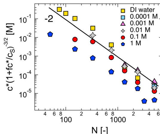
Fig. 16 Overlap concentration of NaPSS in aqueous NaCl solutions, normalised according to eqn (13). Line is power-law of -2 . c^* are calculated using \eta_{sp}(c^*) = 1 criterion using data from ref. 100. A residual salt content of c_s = 7.4 \times 10^{-5} M was assumed. 100
