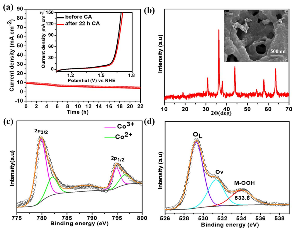
Fig. 8 (a) CA plots with polarisation curves of the fresh and exhausted NiCo 0.5 Fe 1.5 O 4 in the inset; (b) XRD pattern with FE-SEM image of the exhausted NiCo 0.5 Fe 1.5 O 4 ; (c) Co 2p and (d) O 1s spectra of the exhausted NiCo 0.5 Fe 1.5 O 4 .
