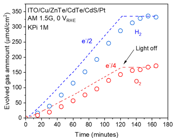
Fig. 10 Hydrogen and oxygen evolution from the ITO/Cu/ZnTe/CdTe/CdS/Pt (RTA) photocathode under simulated sunlight in a three-electrode configuration with an applied potential of 0 V RHE . The expected amounts of hydrogen and oxygen (denoted as e - /2 and e - /4, respectively) as calculated from the observed photocurrent are shown as dashed lines. A 1 M aqueous KPi solution with pH adjusted to 6.5 with KOH was used as the electrolyte.
