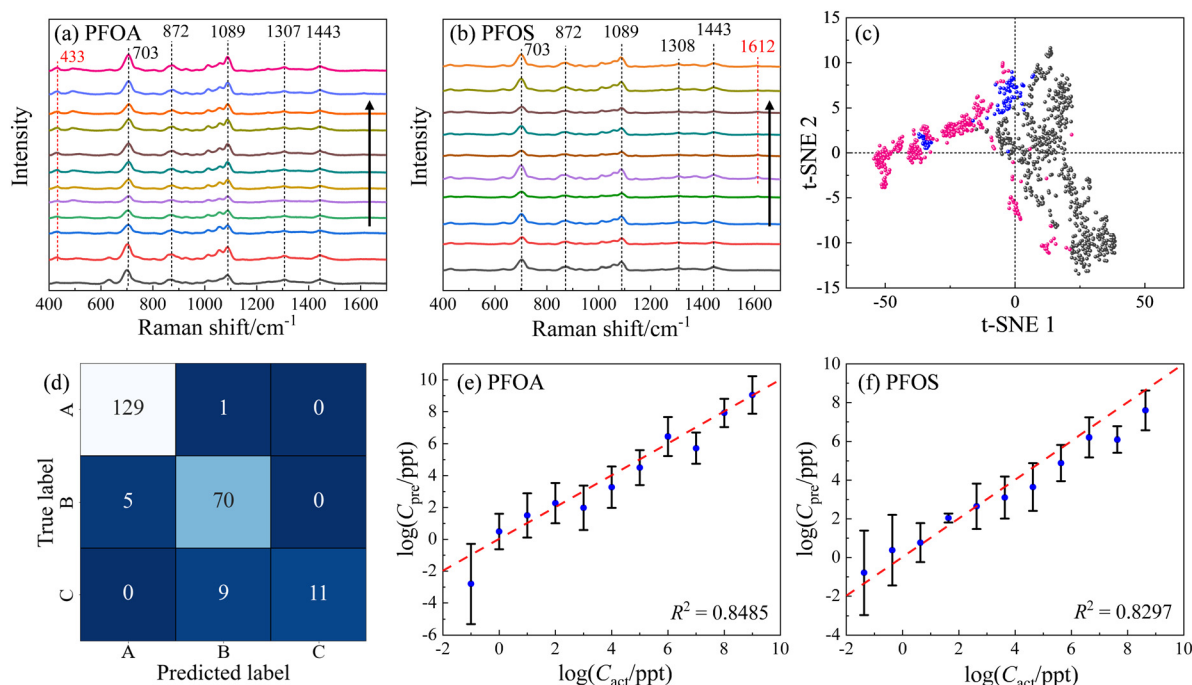
Fig. 6 The average SERS spectra from MCH modified AgNR substrates: (a) PFOA of concentrations of 0, 10^{-1} , 10^0 , 10^1 , 10^2 , 10^3 , 10^4 , 10^5 , 10^6 , 10^7 , 10^8 , and 10^9 ppt, respectively; and (b) PFOS with concentrations of 0, 4.28 \times 10^{-2} , 4.28 \times 10^{-1} , 4.28, 4.28 \times 10^1 , 4.28 \times 10^2 , 4.28 \times 10^3 , 4.28 \times 10^4 , 4.28 \times 10^5 , 4.28 \times 10^6 ppt, respectively. The arrows in the figures indicate the direction of the concentration increase. (c) t -SNE result for PFOS (pink), PFOA (grey), and reference (blue) samples, including spectra from all concentrations. (d) The SVM classification confusion matrix for PFOS, PFOA, and reference samples. A: different concentrations of PFOA; B: different concentrations of PFOS; and C: MCH-modified AgNR substrates. (e) and (f) the log-log plot of C_{pre} versus C_{act} of PFOA and PFOS via two independent SVR models, respectively.
