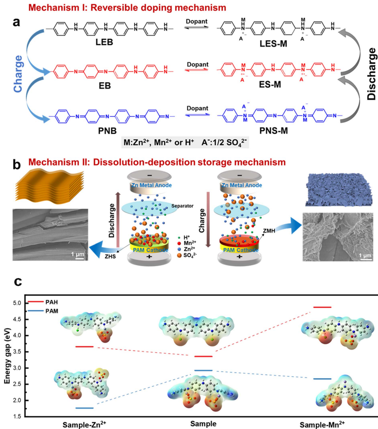
Fig. 7 Schematic diagram of the interactive dual energy storage mechanism of PAM. (a) Mechanism I: reversible doping mechanism of \text{Mn}^{2+} along with \text{H}^{+} and \text{Zn}^{2+} into the conjugated backbone. (b) Mechanism II: dissolution–deposition storage mechanism of \text{Mn}^{2+} on the cathode surface. (c) The plot of energy gap variation for PAH and PAM sample materials doped with \text{ZnSO}_4 and \text{MnSO}_4 electrolytes.
