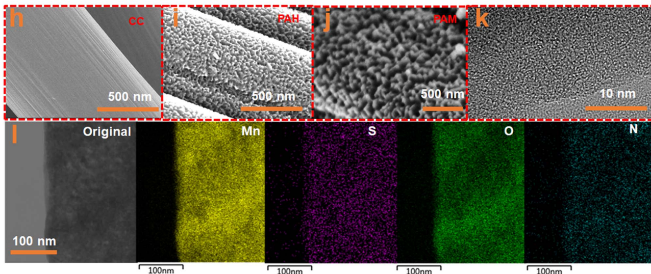
Fig. 1 Synthesis, theoretical modeling and characterization of PANI-based electrodes. (a) Synthesis of H + -doped PANI (PAH) and Mn 2+ -doped PANI (PAM); (b) electrostatic potential (ESP) distribution, (c) calculated energy levels and (d) \pi -electron localization function image of the optimized PAM monomer; (e) XRD patterns, (f) Raman and (g) XPS spectra of PAH and PAM; SEM images of (h) carbon cloth, (i) PAH and (j) PAM; (k) TEM and (l) mapping images of PAM.
