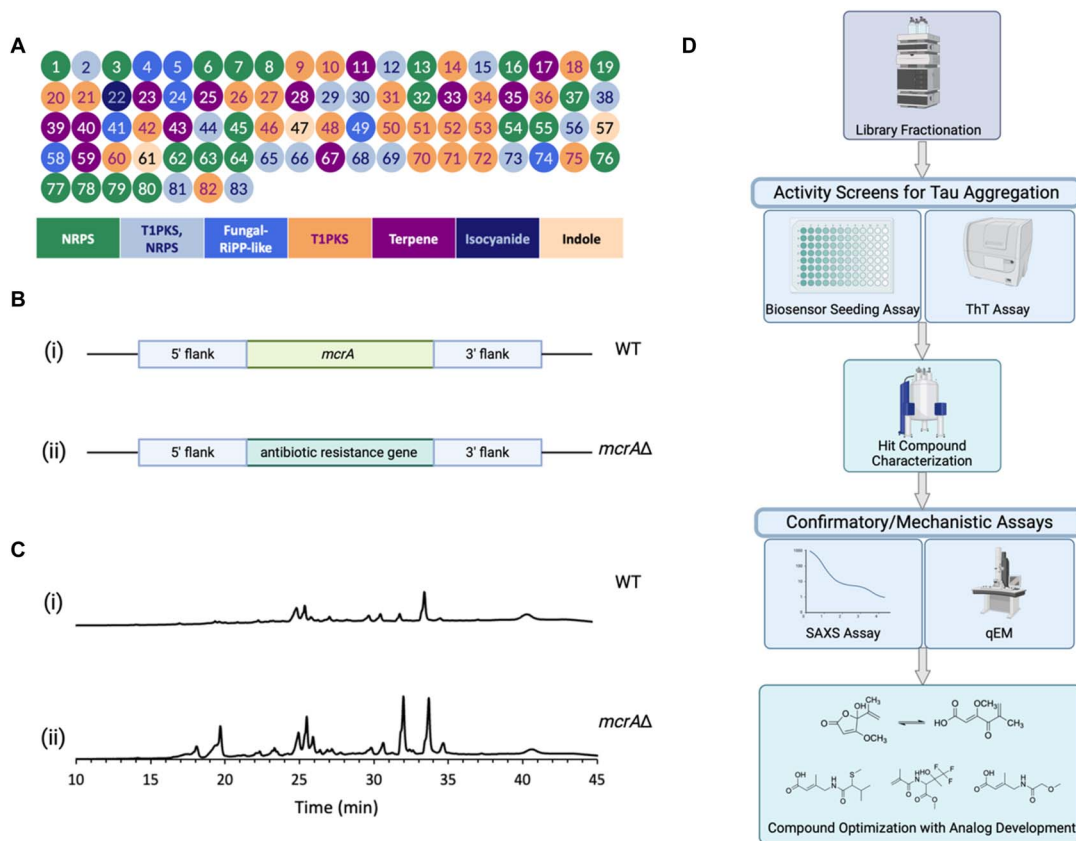
Fig. 1 Activation of silent BGCs that are not expressed under normal laboratory conditions. (A) Predicted BGCs in IMV01140 generated by anti-SMASH. (B) Comparison of (i) WT and (ii) mcrAD strains. (C) HPLC profiles of secondary metabolites produced under malt agar condition in (i) wild type and (ii) mcrAD (library) strain. (D) Workflow of Tauopathies drug discovery from natural product library.
