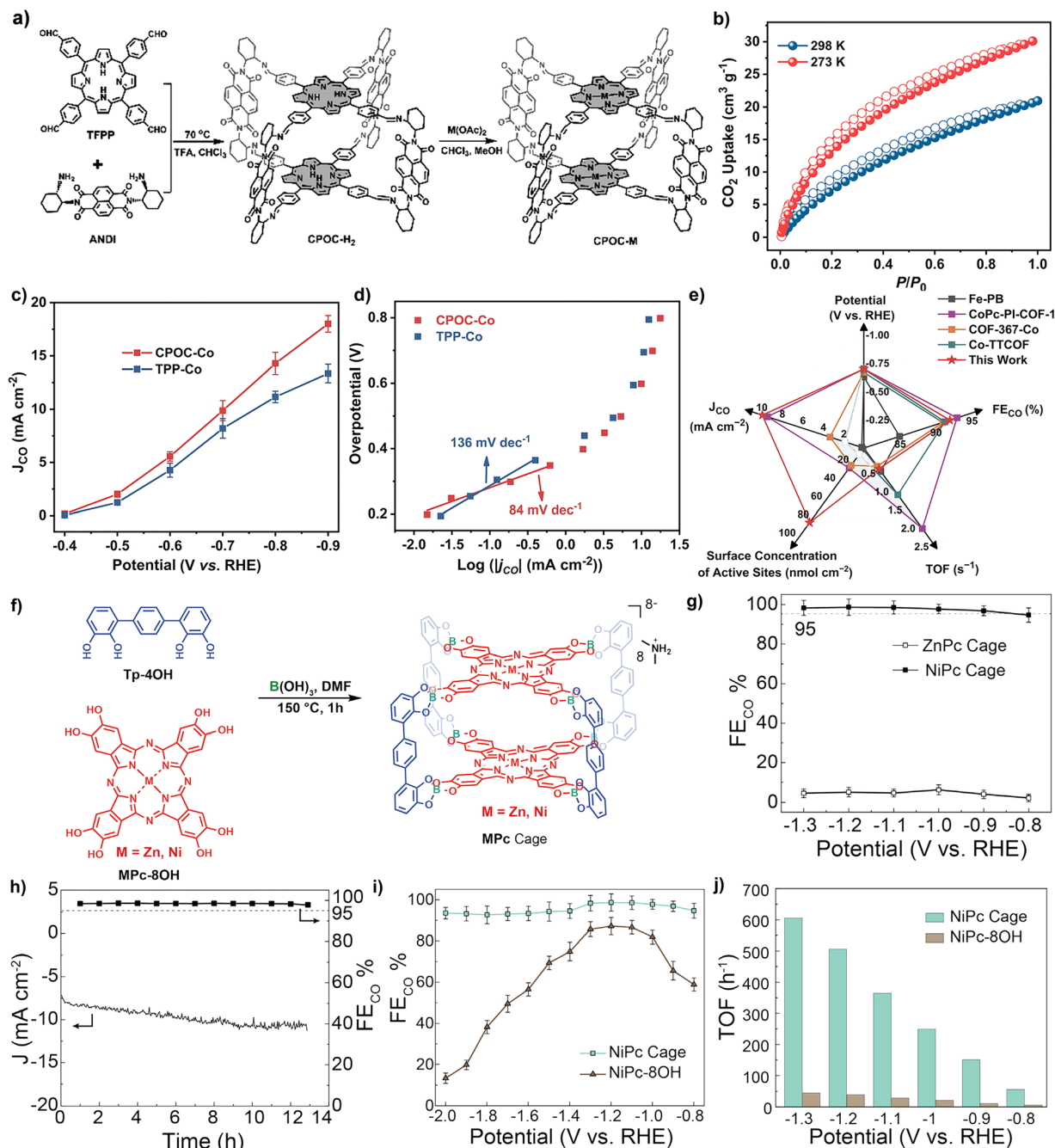
Fig. 5 (a) Schematic synthesis of CPOC-M ( M = H_2, Co(II), Ni(II) ); (b) CO_2 adsorption (solid) and desorption (hollow) curves of POC- H_2 ; (c) comparison of the partial CO current density between CPOC-Co and TPP-Co; (d) Tafel plots of CPOC-Co and TPP-Co; (e) comparison of the performance to that of other materials. Reproduced from ref. 76. Copyright 2023, The Royal Society of Chemistry. (f) Pictorial representation of the formation of an MPc cage; (g) CO faradaic efficiency of ZnPc and NiPc cages; (h) stability test of the NiPc cage at 1.2 V for 13 h; (i) CO faradaic efficiency of the NiPc cage and NiPc-8OH; (j) TOF comparison of the NiPc cage and NiPc-8OH. Reproduced from ref. 77. Copyright 2023, The Cell Press.
