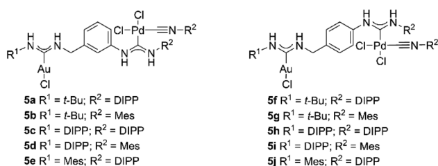
Scheme 4 (a) Previously synthesized isonitrile palladium(II) complexes 4a–b ; (b) previously synthesized heterobimetallic gold(I) palladium(II) complexes 5a–j ; DIPP = 2,6-diisopropylphenyl-, Mes = mesityl-.
