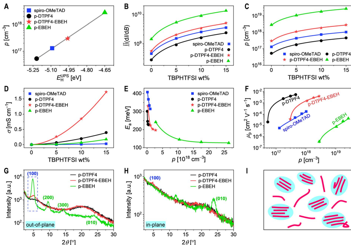
Fig. 2 (A) Semi-logarithmic plot depicting the relationship between hole density ( p ) and the energy levels of HOMO, acquired through ultraviolet photoelectron spectroscopy measurements ( E_H^{UPS} ). The solid gray line represents a linear fit. (B) Semi-logarithmic plots illustrating the quadratic integral of the electron paramagnetic resonance signal ( \int \int (dI/dB) ) as a function of TBPHFISI weight percentage. Linear fits in conventional coordinates are denoted by solid lines. (C) Semi-logarithmic plots displaying the variation of hole density ( p ) with respect to TBPHFISI weight percentage. Linear fits in conventional coordinates are delineated by solid lines. (D) Plots depicting the conductivity ( \sigma ) as a function of TBPHFISI weight percentage. Solid lines represent power-law fits. (E) Plot of activation energy ( E_a ) versus hole density ( p ). Solid lines depict mono-exponential decay fits. (F) Logarithmic plots illustrating the dependence of hole mobility ( \mu_p ) on hole density ( p ). Solid lines serve as visual guide lines. (G and H) Out-of-plane and in-plane grazing-incidence X-ray diffraction patterns of conjugated polymer thin films on monocrystalline silicon substrates. (I) Schematic representation elucidating the microstructure of p-EBEH thin film, where crystalline regions are discontinuous.
