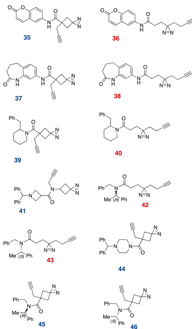
Fig. 7 Diazirine probes used for live cell labeling.
