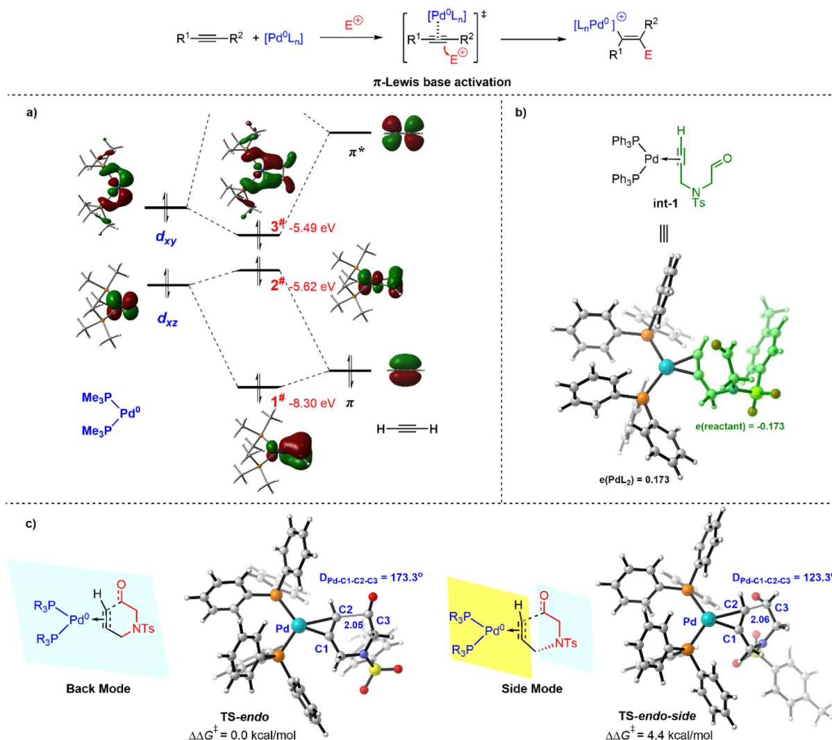
Fig. 1 Pd(0)- \pi -Lewis base activation of alkynes. (a) Molecular orbital analysis for Pd(0) and alkyne. (\text{Me}_3)_2\text{Pd}^0 and acetylene were employed as a simplified model. (b) Mulliken charge distribution of \eta^2 -coordinated Pd(0)-alkynal complex. (c) Comparison of back and side modes for \pi -Lewis base activation.
