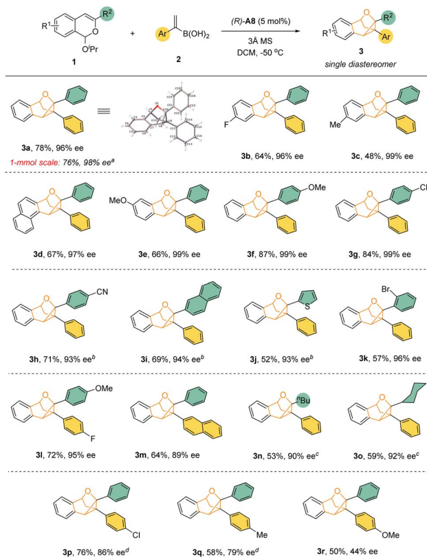
Scheme 2 Reaction scope. Reaction conditions: 1 (0.30 mmol), 2a (0.75 mmol), ( R )- A8 (0.015 mmol), 3 Å MS (30 mg), solvent (1.5 mL), -50^{\circ}\text{C} , 96 h. Isolated yield is provided. The ee value was determined by chiral HPLC analysis. a 168 h. b 10 mol% of catalyst at -35^{\circ}\text{C} . c 10 mol% of catalyst at room temperature for 48 h. d Room temperature.
