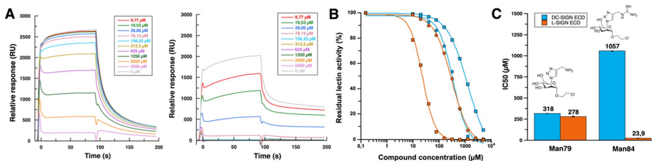
Fig. 3 (A) Sensorgrams of DC-SIGN binding inhibition (left panel) and L-SIGN binding inhibition (right panel) by Man84. Range of Man84 concentrations goes from 5 mM to 10 \mu\text{M} by serial dilution by a factor of 2 with same color code for both DC-SIGN and L-SIGN inhibition. (B) SPR inhibition curves for Man79 (circle) and Man84 (square) (see ESI† for all sensorgrams). Inhibition curves concerning DC-SIGN are represented in blue and L-SIGN in orange. Man79 data, were already described in Pollastri et al. , 34 and are shown here for direct comparison with Man84 data. (C) \text{IC}_{50} values of Man79 and Man84 for DC-SIGN (in blue) and L-SIGN (in orange). Values represented are the corresponding \text{IC}_{50} .
