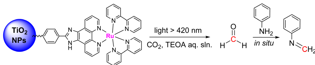
Scheme 50 Visible light reduction of \text{CO}_2 into formaldehyde followed by in situ condensation with an amine. 194
