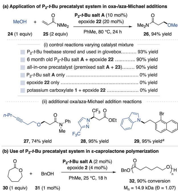
Fig. 6 Use of P_2 - t -Bu salt A in catalytic (a and b) and stoichiometric (c and d) reaction applications. Yields determined by 1 H NMR spectroscopy. a Reaction run in DMSO. b Reaction run in THF. c Preactivation at 100 °C for 1 h in PhMe. d Yields of reactions setup using commercial P_2 - t -Bu in a nitrogen-filled glovebox are provided for comparison.
