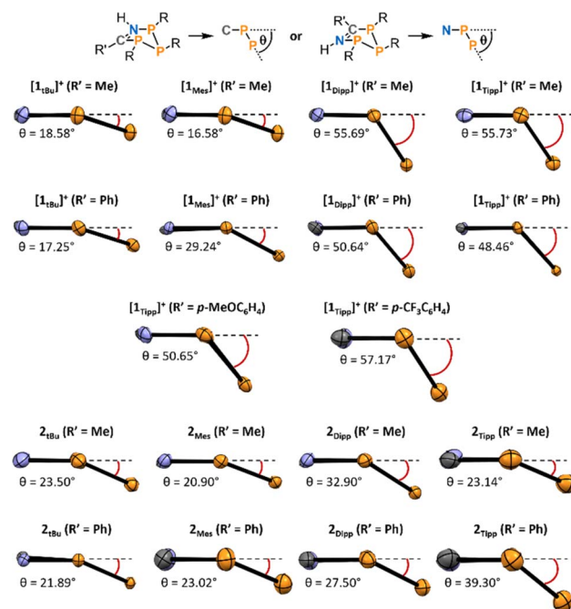
Fig. 4 Side-on view of the central P_3CN rings in the molecular structures as determined by SC-XRD experiments of [1_R]^+ and 2_R demonstrating the angle of bending of each species ( P = orange , C = grey , N = blue ). View was chosen such that the bent-out-of-plane P_P atom sits to the right, and all \theta values are measured from the horizontal P_C-C=N-P_N plane (represented as a dotted line parallel to the bottom of the page) downward to the plane formed by the three phosphorus atoms. Thermal ellipsoids are drawn at the 50% probability level.
