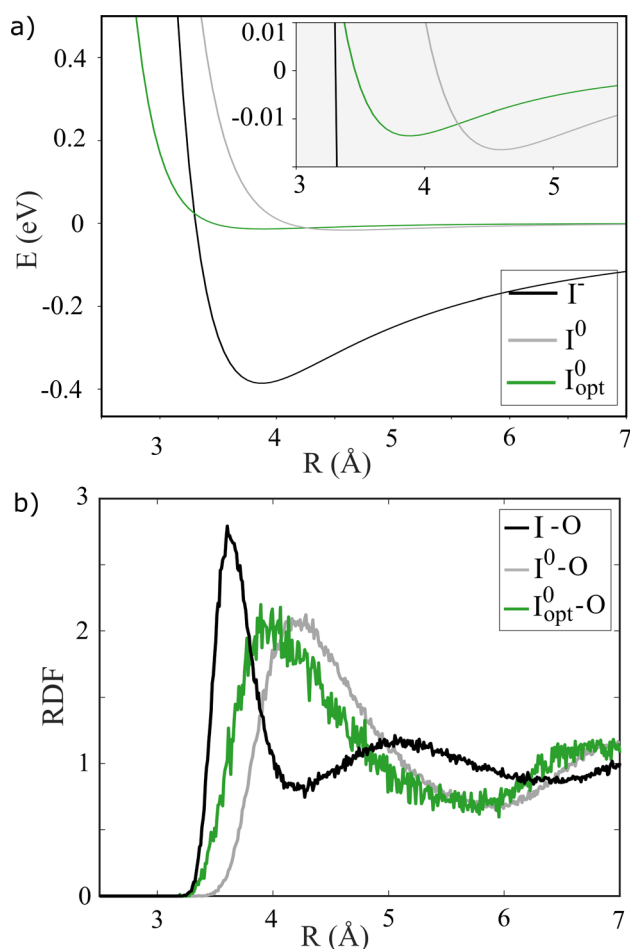
Fig. 3 (a) Iodide/dine-water dimer potential curves based on the dimer geometry determined in Fig. S3 in the ESI,† calculated using iodide and the excited state iodine with ( \text{I}^0_{\text{opt}} ) and without ( \text{I}^0 ) optimized parameters. (b) RDFs calculated by classical MD simulation for the halide-oxygen distance of aqueous NaI.
