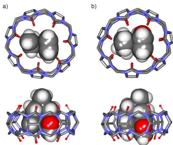
Fig. 5 Energy-minimized structures at the PM6 level of theory of 1 : 1 inclusion complexes: (a) FA-1@CB[7] (bottom view and side view), and (b) FA-2@CB[7] (bottom view and side view). CB[7] is shown in line-stick representation with non-polar hydrogen atoms omitted for clarity. Bound guests are depicted as CPK models. See Fig. 1 for the line-drawing structures of the compounds.
