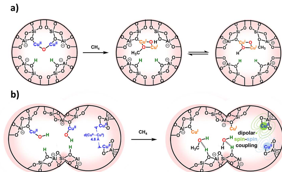
Fig. 14 Suggested reaction pathways of Cu–O species in Cu-MOR and their transformations during the reaction with CH 4 . (a) Pathway involving [\text{Cu}_2(\mu\text{-O})]^{2+} species. (b) Pathway involving [\text{CuOH}]^+ species, highlighting the inactivity of monomeric Cu species exhibiting dipolar spin–spin coupling at a separation distance of 4.8 Å.
