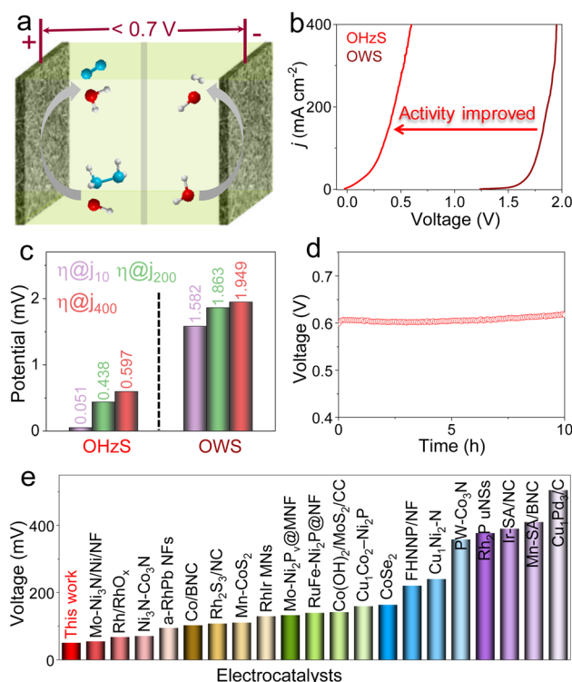
Fig. 5 (a) Schematic illustration of two-electrode OHZS electrolyzer constructed by \text{Fe-Ni}_2\text{P/CeO}_2 . (b) OWS and OHZS polarization curves for \text{Fe-Ni}_2\text{P/CeO}_2 and (c) corresponding voltage comparison at 10, 200 and 400 \text{ mA cm}^{-2} . (d) Stability test for \text{Fe-Ni}_2\text{P/CeO}_2 at a constant current density of 400 \text{ mA cm}^{-2} in 1.0 M KOH with 0.5 M \text{N}_2\text{H}_4 . (e) Comparison of OHZS performances of \text{Fe-Ni}_2\text{P/CeO}_2 with those of other developed catalysts.
