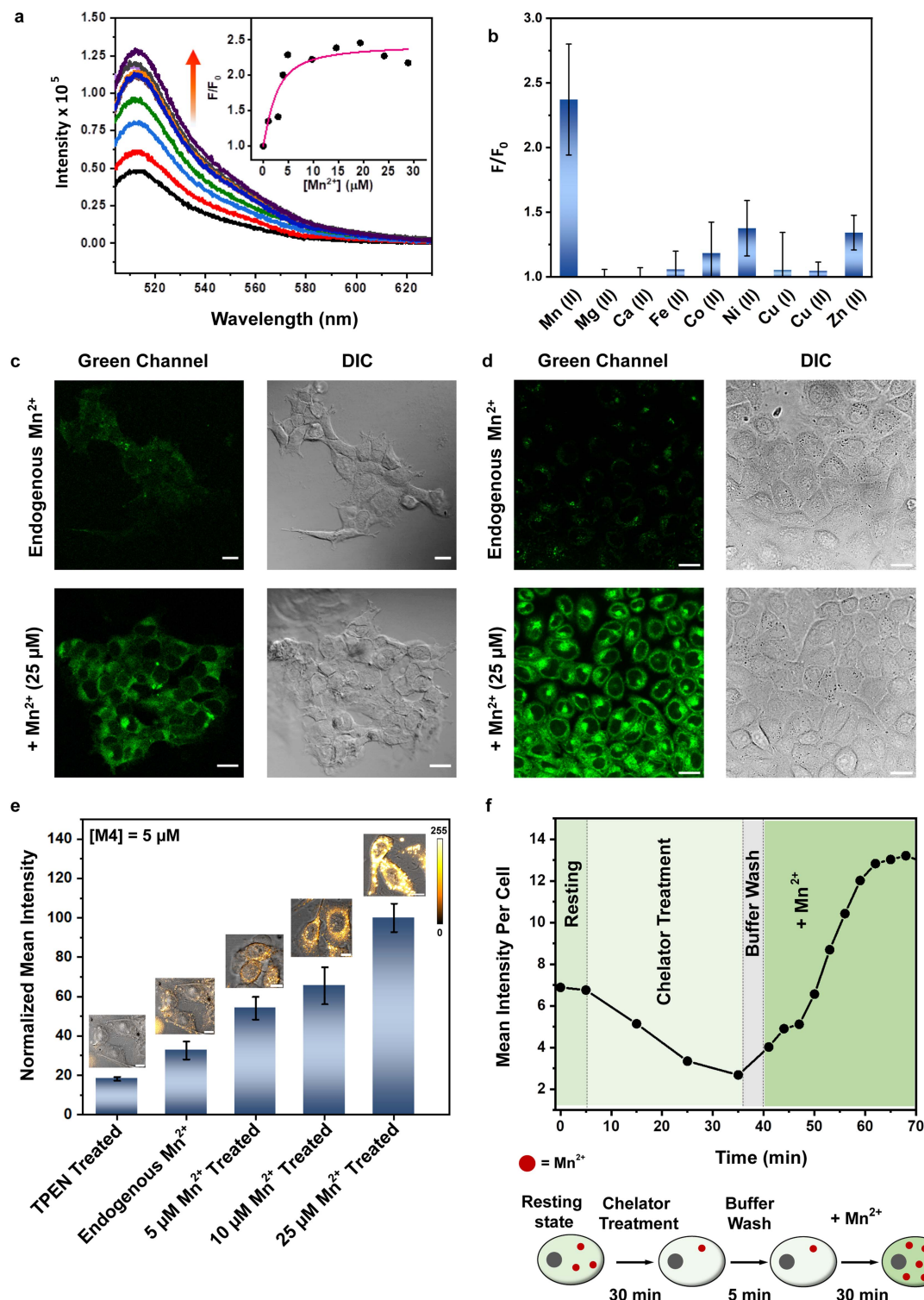
Fig. 3 Visualizing and quantifying endogenous labile Mn^{2+} in mammalian cells. (a) Fluorescence response of M4 (2 \mu M ) to Mn^{2+} (0 \mu M to 28 \mu M ) in HEPES (20 mM) and KNO_3 (100 mM) buffer (pH 7.1), \lambda_{ex} 480 nm. Inset: Observed fluorescence intensity ( F ) over initial fluorescence intensity in the absence of Mn^{2+} ( F_0 ) at 514 nm over an Mn^{2+} ion concentration range of 0–28 \mu M (black circles; the red line is the fitted curve). (b) Observed fluorescence intensity ( F ), in the presence of different biologically relevant metal ions, including Mn^{2+} ( [M^{n+}] = 15 \mu M ), over initial fluorescence intensity in the absence of any metal ion ( F_0 ) at 514 nm. Data are presented as SEM where n = 3 in each set. (c) Representative confocal single z plane images of HEK293T cells. Cells were incubated with: M4 (5 \mu M ) in aqueous buffer (pH 7.4) for 15 min (upper panel); with 25 \mu M Mn^{2+} in aqueous buffer (pH 7.4) for 1 h, washed and then incubated with M4 in aqueous buffer (pH 7.4) for 15 min (lower panel). Both the sets were washed with aqueous buffer (pH 7.4) and imaged; differential interference contrast (DIC) images are in the right columns for the respective confocal images. Scale bar = 20 \mu m . (d) Representative confocal single z plane images of HeLa cells. Cells were incubated with: M4 (5 \mu M ) in aqueous buffer (pH 7.4) for 15 min (upper panel); with 25 \mu M Mn^{2+} in aqueous buffer (pH 7.4) for 1 h, washed and then incubated with M4 in
