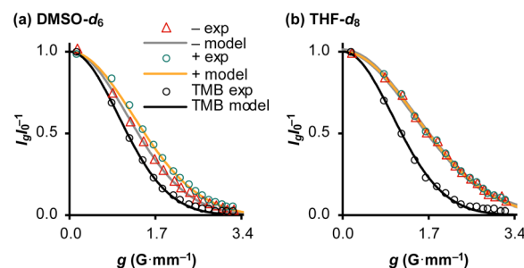
Fig. 2 Diffusion profiles of \text{Ph}_3\text{SiF}_2^- (“-”), {}^n\text{Bu}_4\text{N}^+ (“+”) and the internal diffusion standard (“TMB”) in: (a) 1.5 mM TBAT and 263 mM TMB in DMSO- d_6 , and (b) 207 mM TBAT and 252 mM TMB in THF- d_8 ; both at 300 K.
