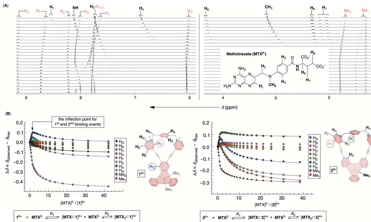
Fig. 5 (A) Segment of ^1\text{H} NMR spectra of 47\ \mu\text{M}\ 1^{6+} in water (30 mM PBS buffer at pH = 7.4) obtained after incremental addition of 2.5 mM solution of \text{MTX}^{2-} . (B) A relative change of the chemical shift of protons from 1^{6+} (left) or 2^{6+} (right) was fit to 1 : 2 model describing the formation of binary [\text{MTX}\subset 1]^{4+} and ternary [\text{MTX}_2\subset 1]^{2+} complexes.
