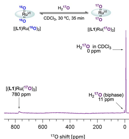
Fig. 8 ^{17}\text{O} NMR spectrum of [(\text{L1})\text{Ru}^{\text{VI}}(^{16}\text{O})_2] with ^{17}\text{OH}_2 in \text{CDCl}_3 .
