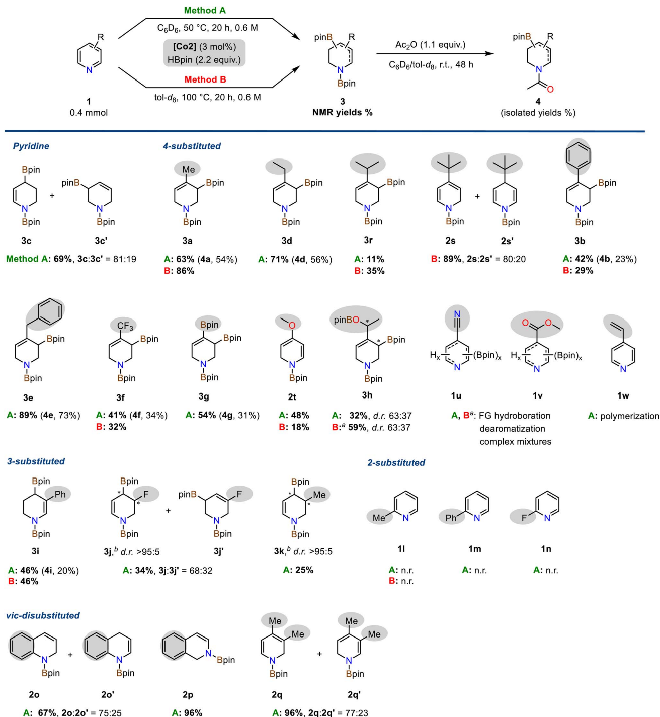
Scheme 3 Substrate scope of the double hydroboration of pyridines. Conditions: Pyridine (0.40 mmol), HBpin (0.88 mmol, 2.2 equiv.), Co 2 (3 mol%) in C 6 D 6 at 50 °C (Method A) or in tol- d 8 at 100 °C (Method B) at 0.6 M for 20 h inside a headspace vial (5 mL) with magnetic stirring unless otherwise specified. Yields of di-boryl products (shown in bold) were determined by 1 H-NMR spectra of the crude mixtures vs. internal hexamethylbenzene (Method A) or 1,3,5-trimethoxybenzene (Method B). Isolated yields of the N -acetyl allyl boronates given in parentheses. a 4.4 equiv. HBpin. b Only a single diastereomer observed in 1 H-NMR spectra. n. r. = no reaction.
